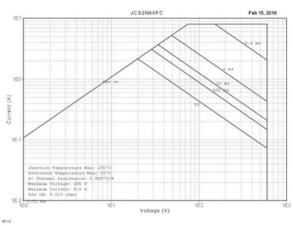
Maximum Safe Operating Area For JCS2N60FC(TO-220MF)
